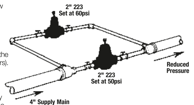
Fig. 4 – Parallel Installation
